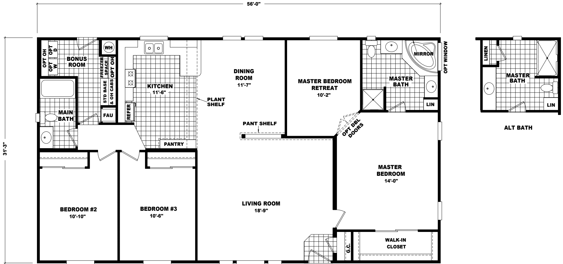
MODEL : XL-3256D APPROXIMATELY 1750 SQ. FT. 3 BEDROOM, 2 BATH
