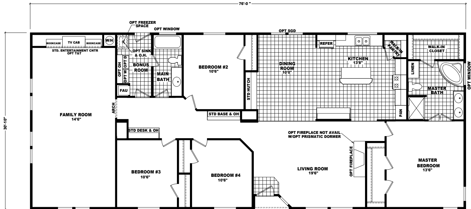
MODEL: WLS-3276B APPROXIMATELY 2343 SQ. FT. 4 BEDROOM, 2 BATH
