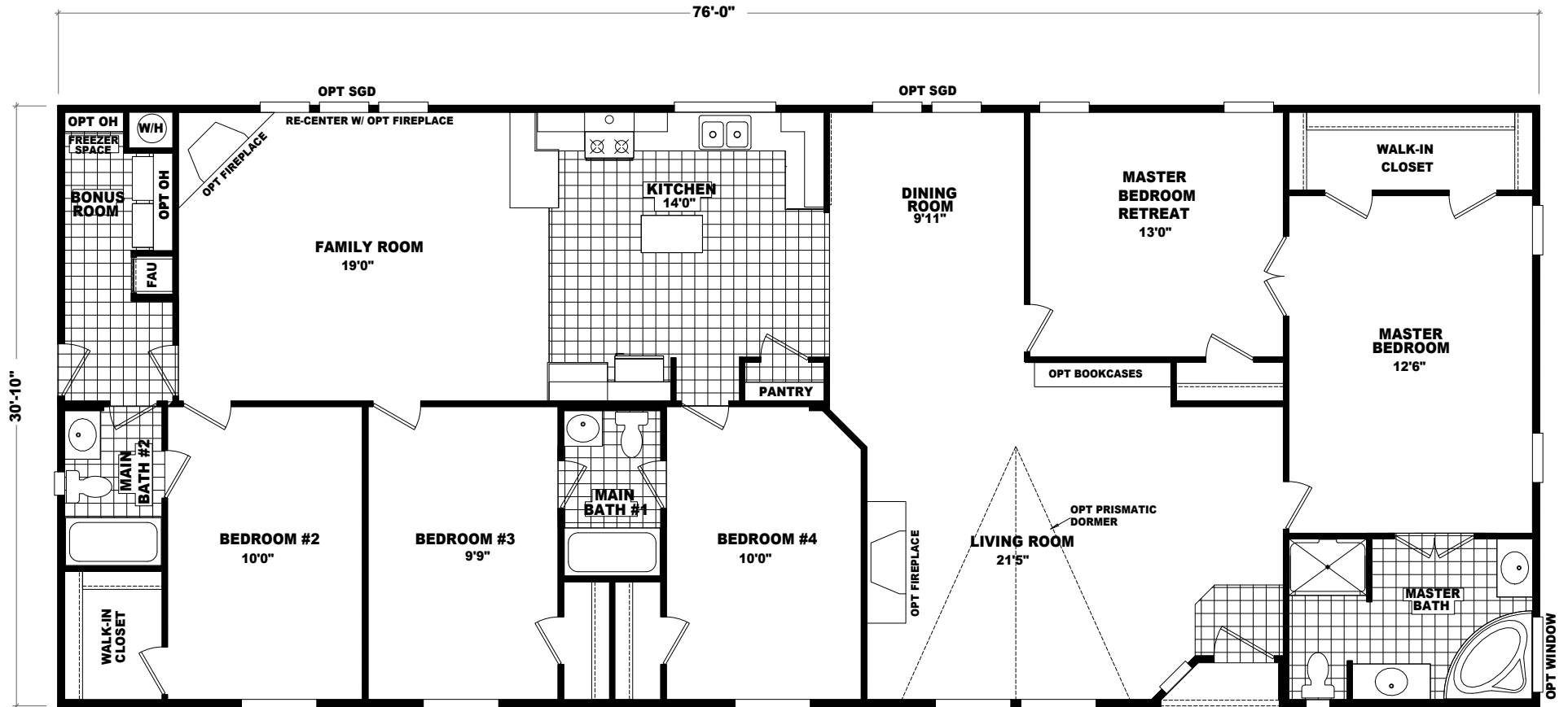
MODEL: WLS-3276A APPROXIMATELY 2343 SQ. FT. 4 BEDROOM, 3 BATH
