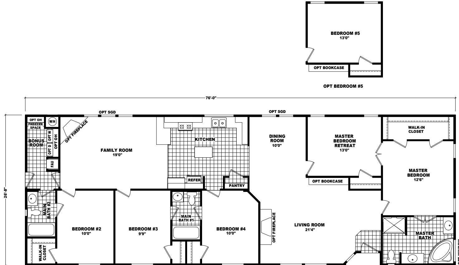
MODEL: WLS-2876A APPROXIMATELY 2022 SQ. FT. 4 BEDROOM, 3 BATH
