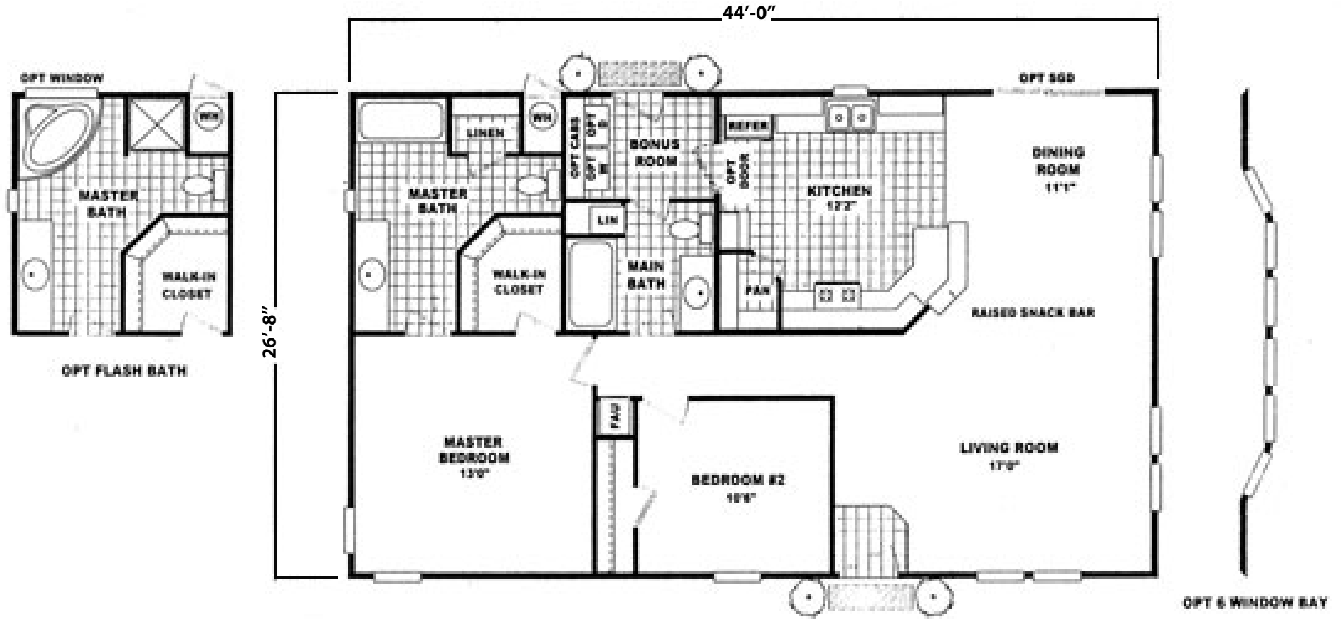
MODEL: VSX-2844B APPROXIMATELY 1173 SQ. FT. 2 BEDROOM, 2 BATH
