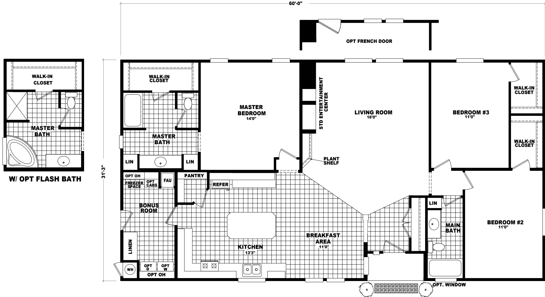
MODEL: VPS-6032A APPROXIMATELY 1875 SQ. FT. 3 BEDROOM, 2 BATH
