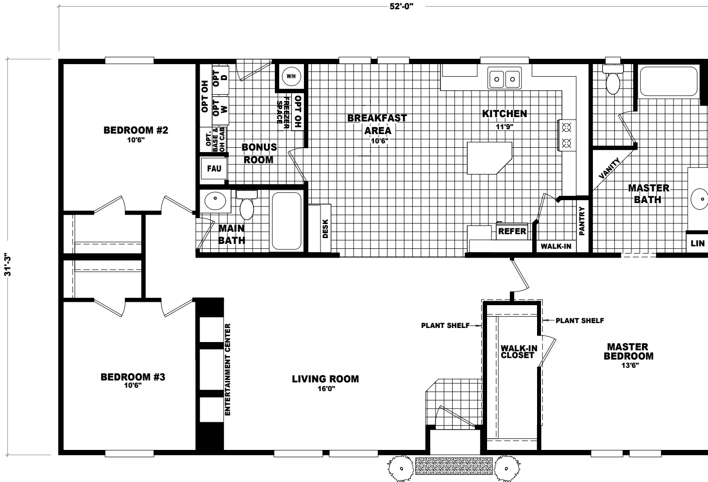
MODEL: VPS-5232A APPROXIMATELY 1625 SQ. FT. 3 BEDROOM, 2 BATH
