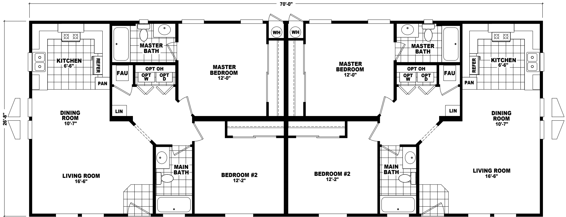
UNIT-B APPROXIMATELY 933 SQ. FT. 2 BEDROOM, 2 BATH
