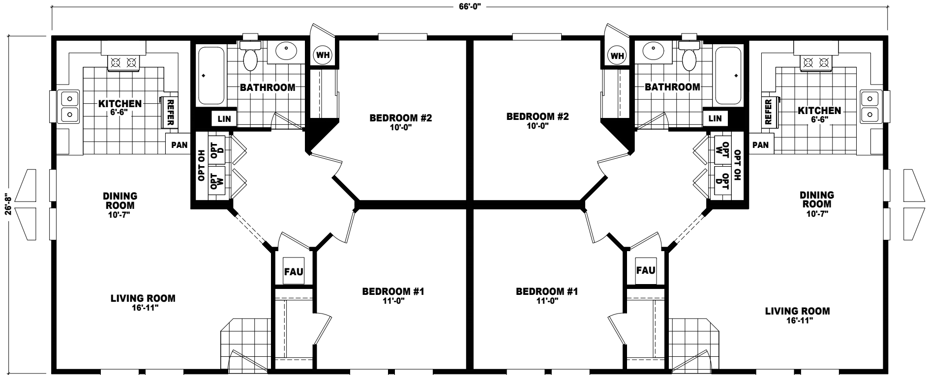
UNIT-B APPROXIMATELY 880 SQ. FT. 2 BEDROOM, 1 BATH
