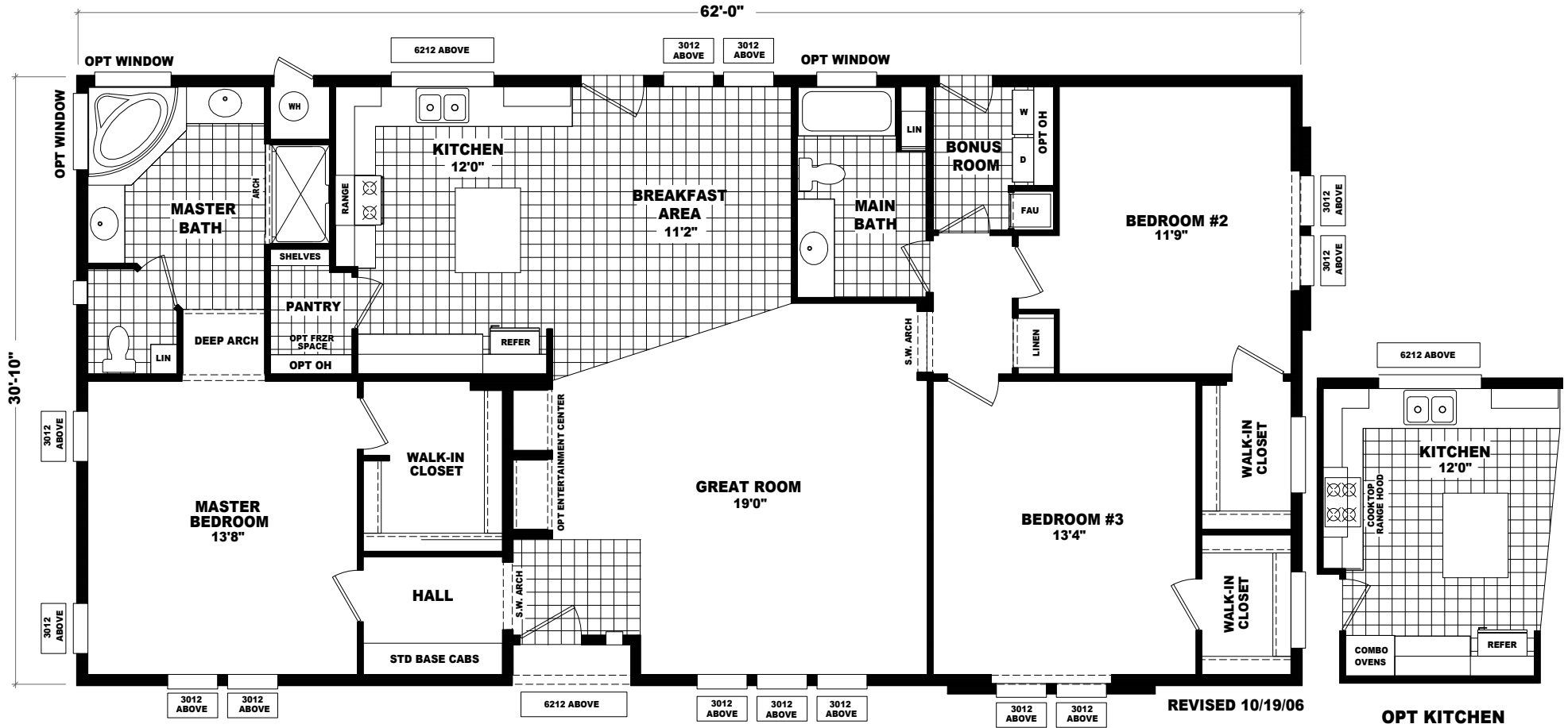
MODEL: TR1912A APPROXIMATELY 1912 SQ. FT. 3 BEDROOM, 2 BATH
