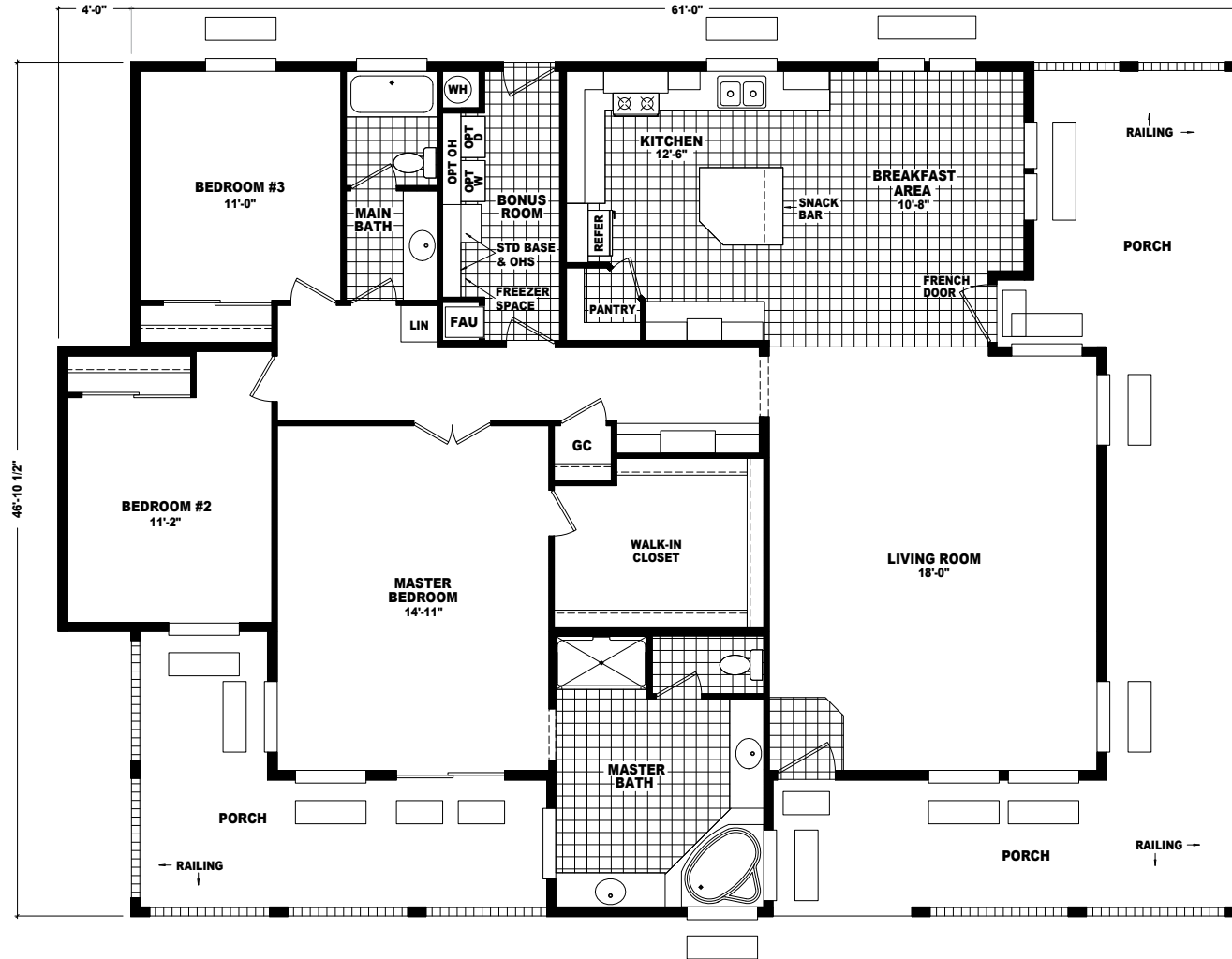
MODEL: STF-2921A APPROXIMATELY 2921 SQ. FT.* 3 BEDROOM, 2 BATH *INCLUDES PORCHES
