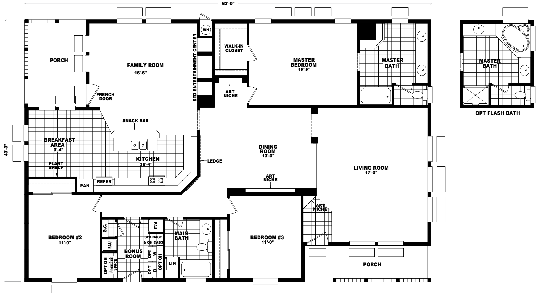
MODEL: STF-2480A APPROXIMATELY 2480 SQ. FT.* 3 BEDROOM, 2 BATH * INCLUDES PORCHES
