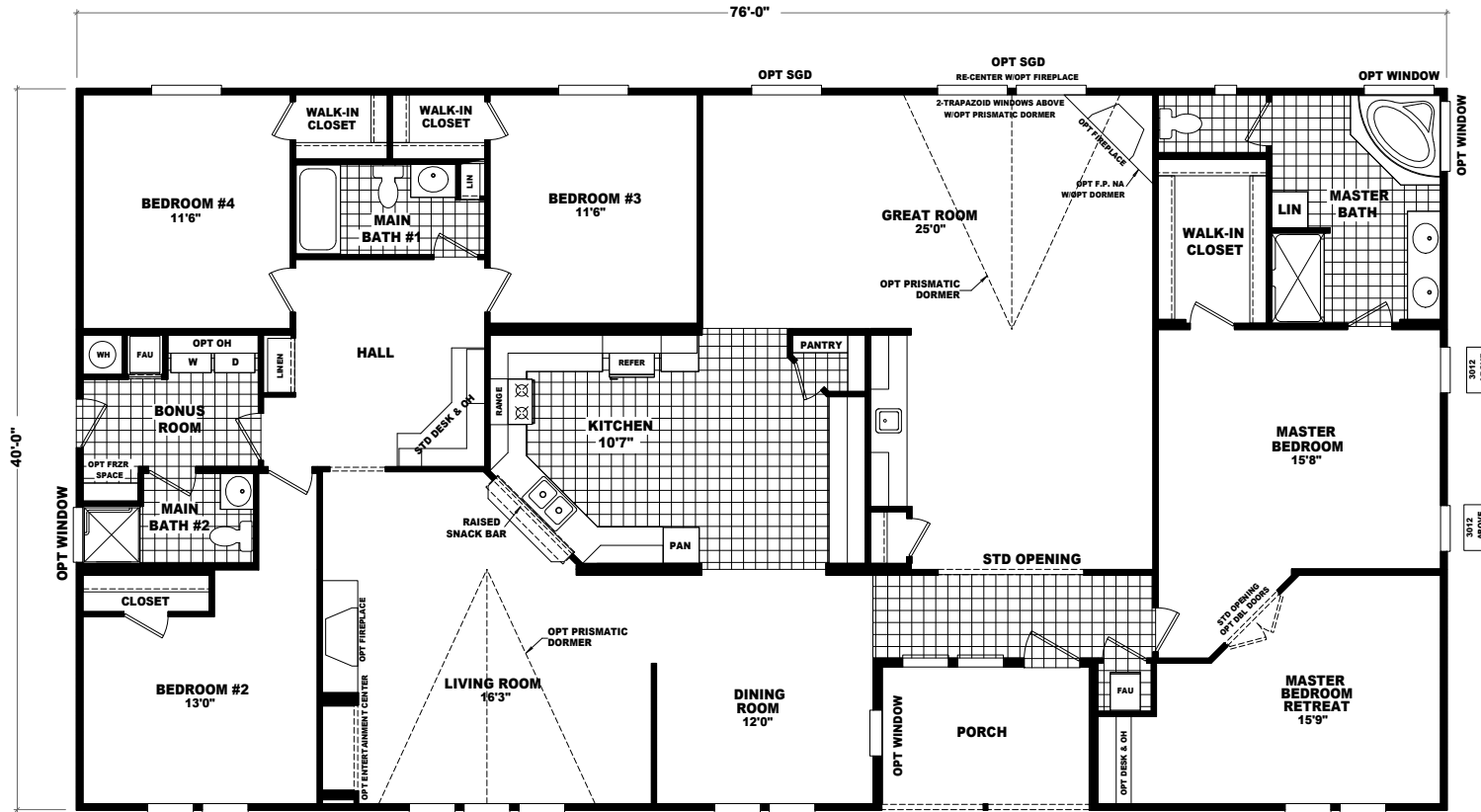
MODEL: LSP3040A APPROXIMATELY 3040 SQ. FT. 4 BEDROOM, 3 BATH
