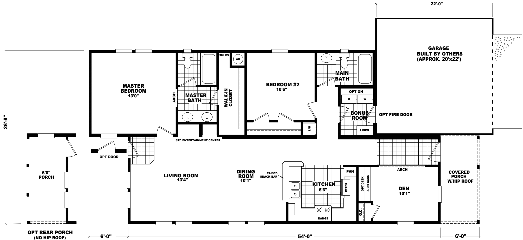
MODEL: LSP-2854H APPROXIMATELY 1226 SQ. FT. 2 BEDROOM, 2 BATH
