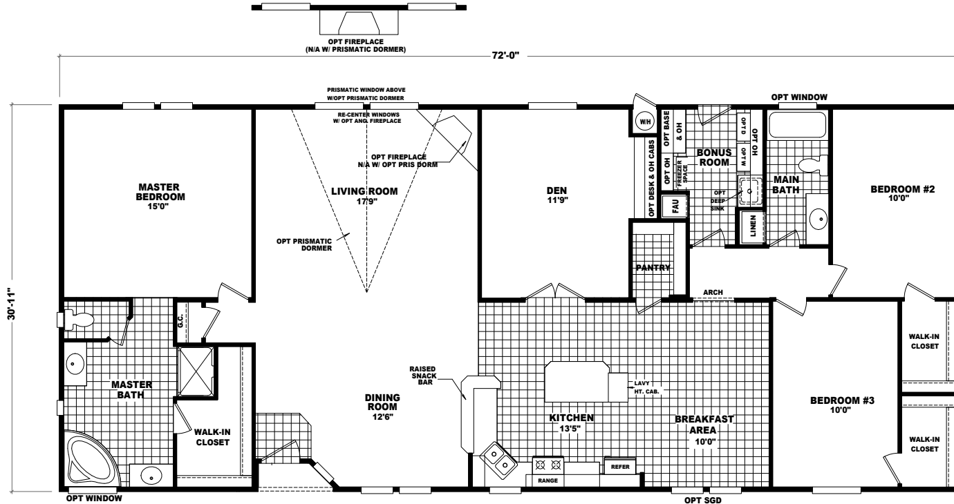
MODEL: LS-3272B APPROXIMATELY 2214 SQ. FT. 3 BEDROOM, 2 BATH
