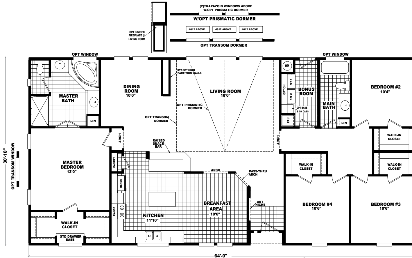
MODEL: LS-3264V APPROXIMATELY 1972 SQ. FT. 4 BEDROOM, 2 BATH
