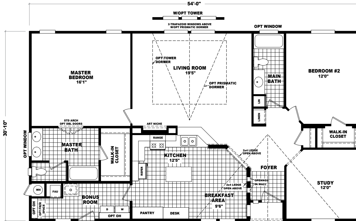
MODEL: LS3254V APPROXIMATELY 1649 SQ. FT. 2 BEDROOM, 2 BATH
