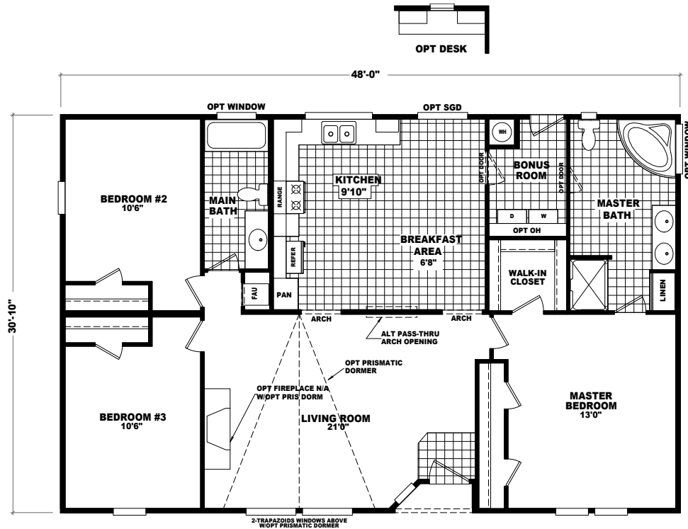
MODEL: LS-3248J APPROXIMATELY 1473 SQ. FT. 3 BEDROOM, 2 BATH
