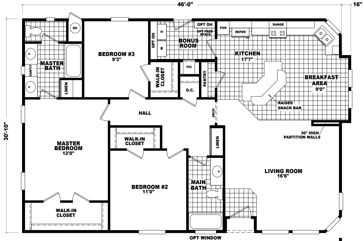
MODEL: LS-3246V APPROXIMATELY 1417 SQ. FT. 3 BEDROOM, 2 BATH
