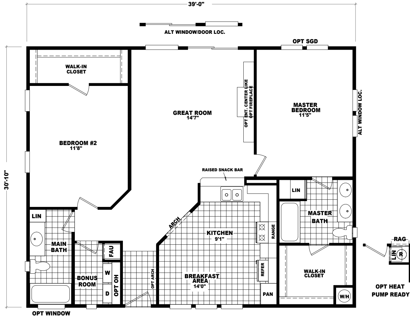
MODEL: LS-3239A APPROXIMATELY 1202 SQ. FT. 2 BEDROOM, 2 BATH
