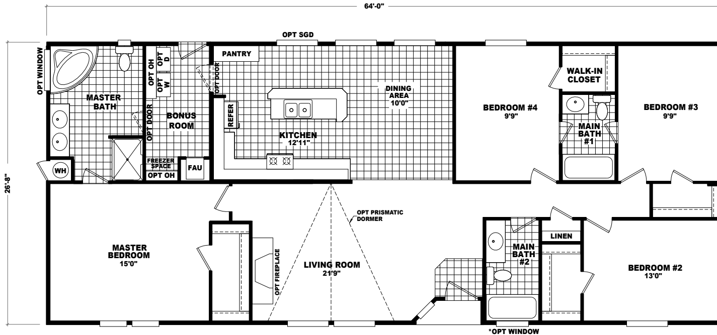
MODEL: LS-2864E APPROXIMATELY 1706 SQ. FT. 4 BEDROOM, 3 BATH
