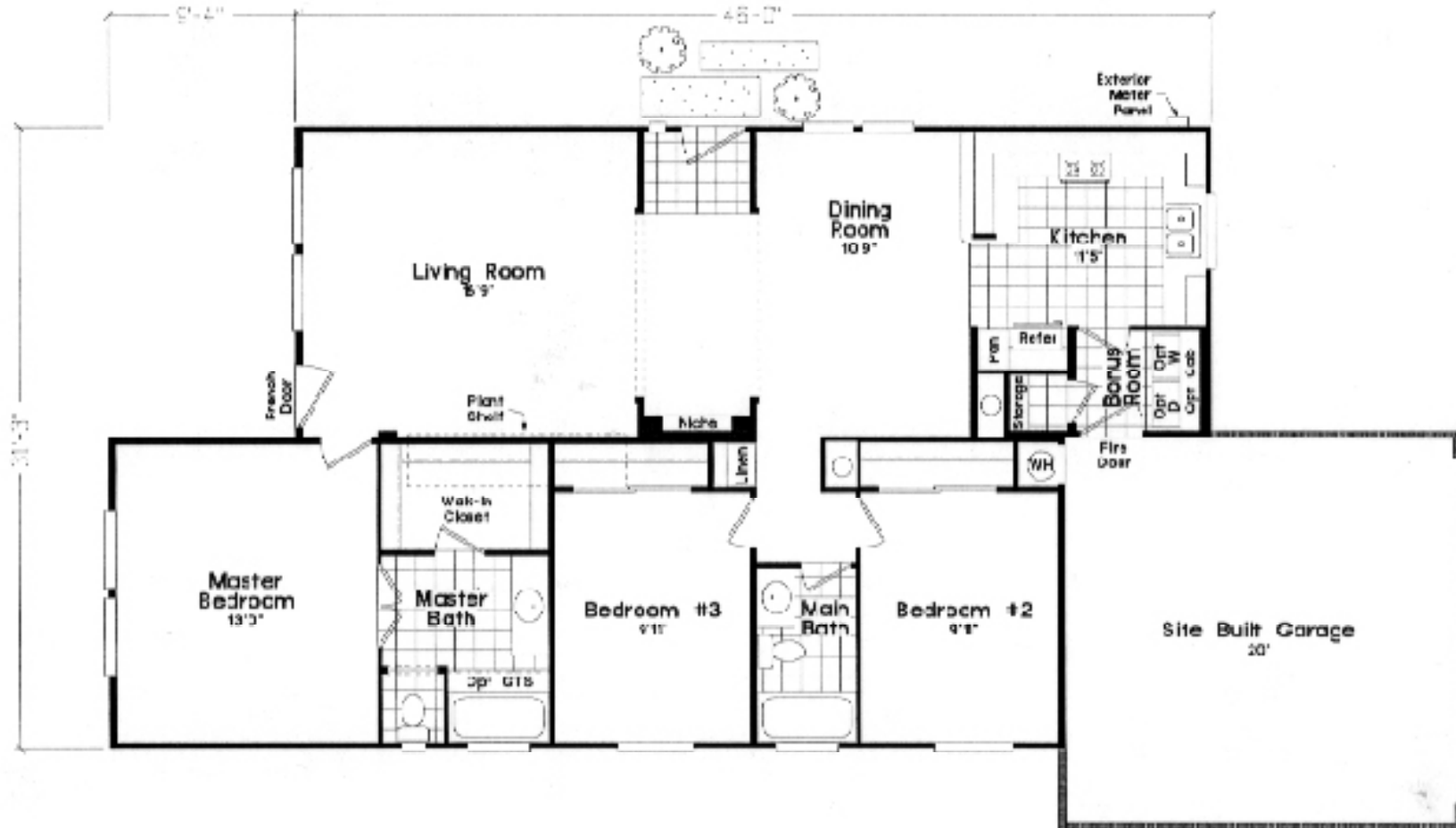
MODEL: HUD/UBC-1468A Approximately 1463 Sq. Ft. 3 Bedroom, 2 Bath
