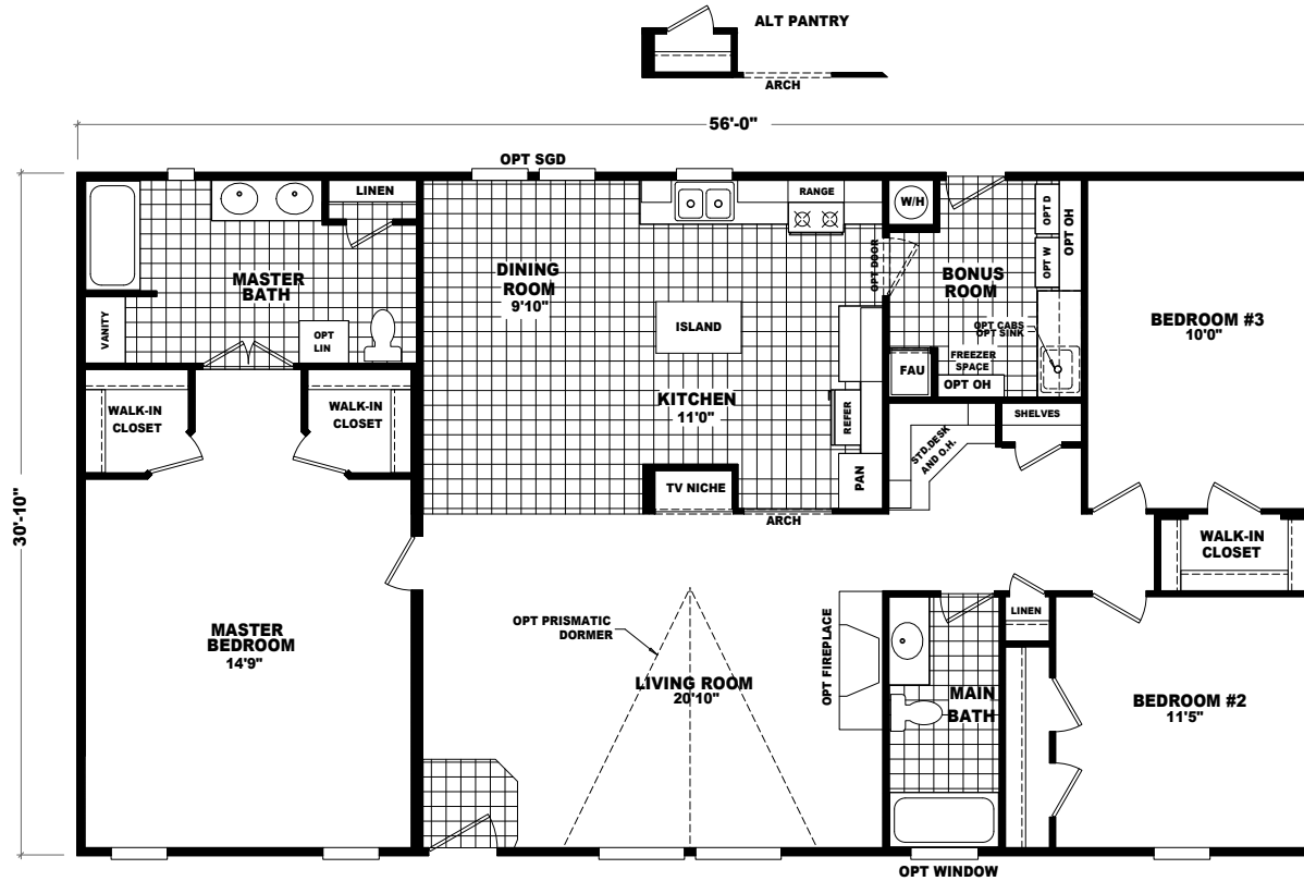
MODEL: GS-3562G APPROXIMATELY 1726 SQ. FT. 3 BEDROOM, 2 BATH
