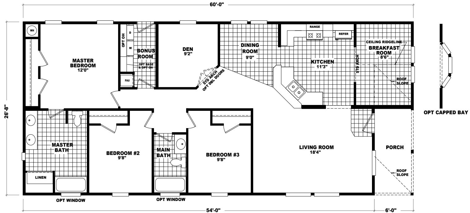
MODEL: GS2608HR APPROXIMATELY 1520 SQ. FT. 3 BEDROOM, 2 BATH
