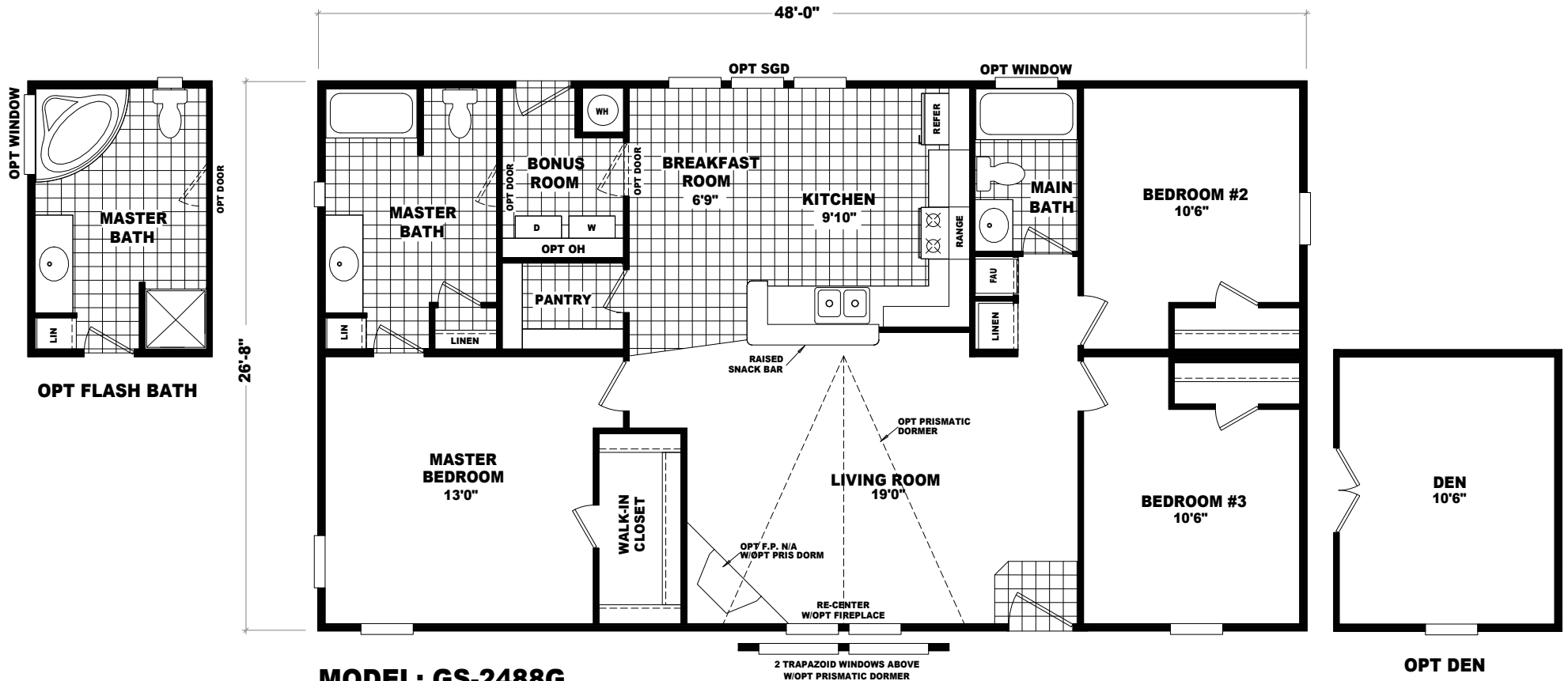
MODEL: GS-2488G APPROXIMATELY 1280 SQ. FT. 3 BEDROOM, 2 BATH
