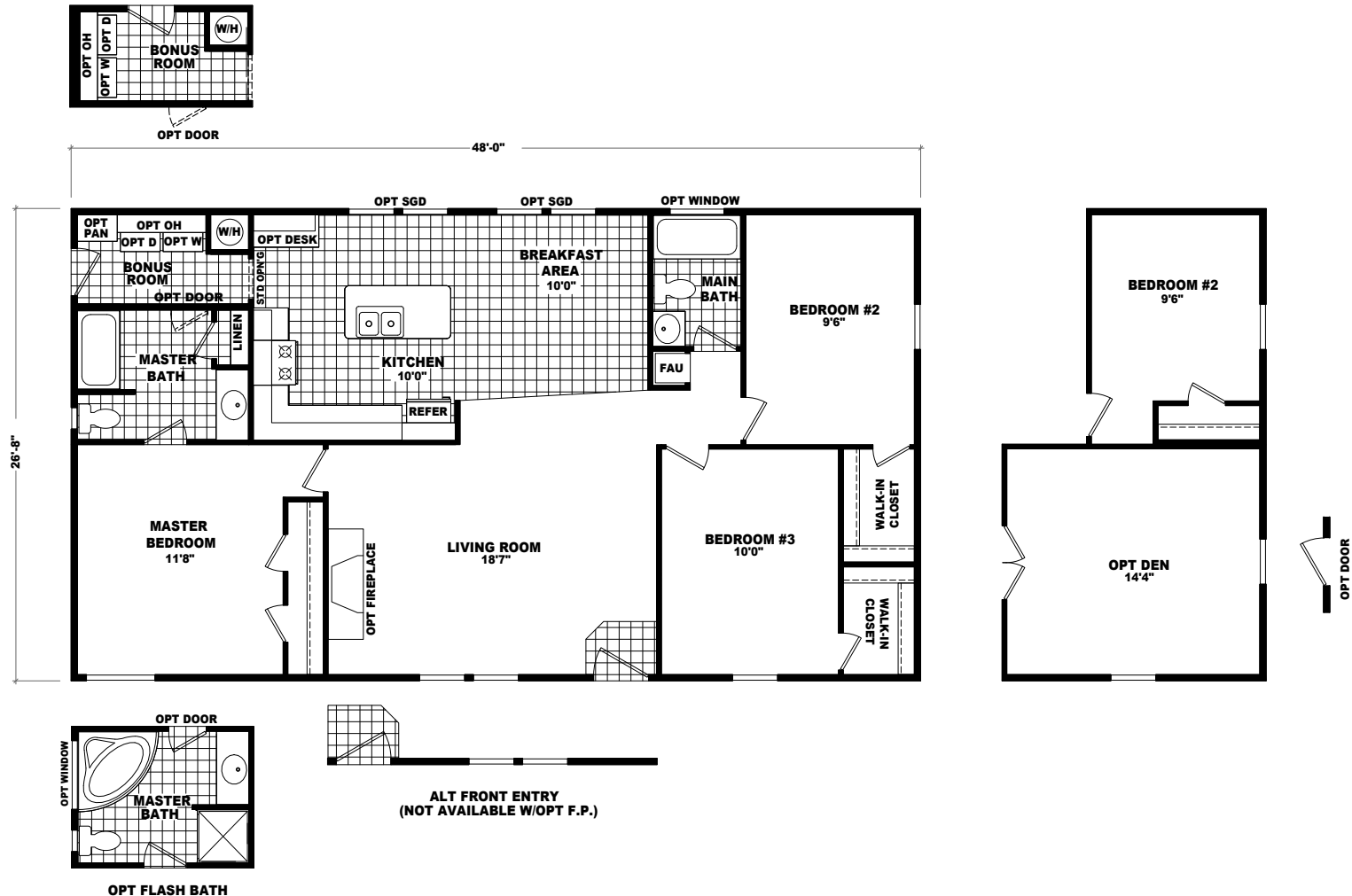
MODEL: GS-2488A APPROXIMATELY 1280 SQ. FT. 3 BEDROOM, 2 BATH
