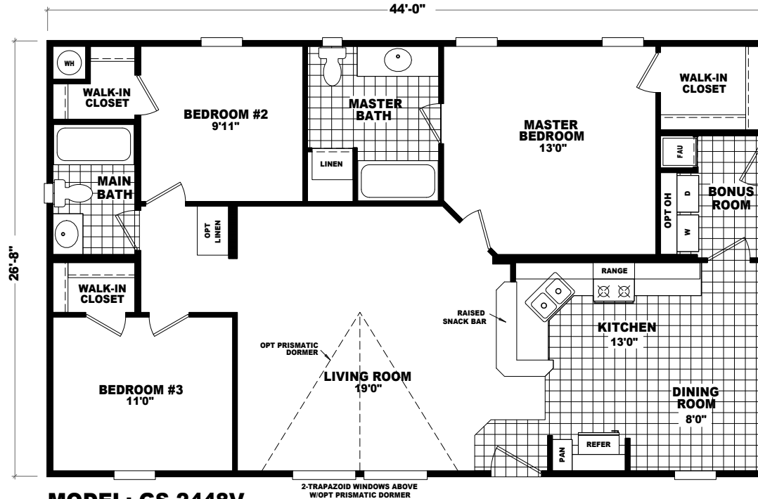
MODEL: GS-2448V APPROXIMATELY 1173 SQ. FT. 3 BEDROOM, 2 BATH
