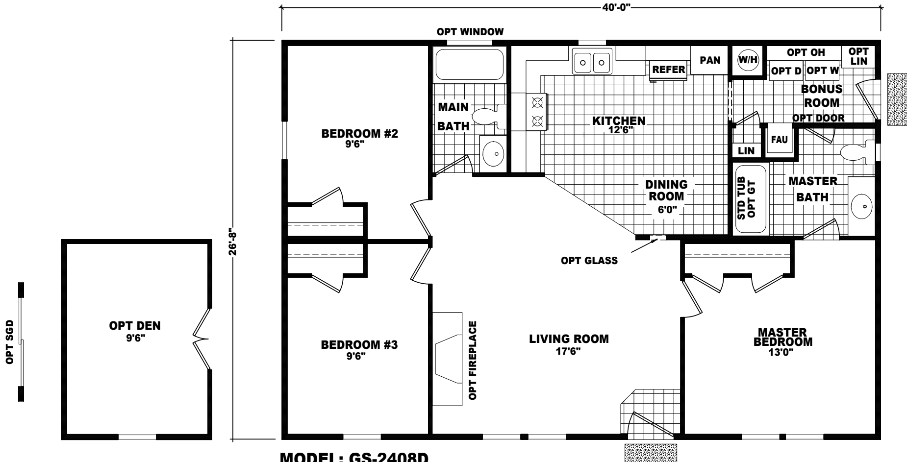
MODEL: GS-2408D APPROXIMATELY 1066 SQ. FT. 3 BEDROOM, 2 BATH
