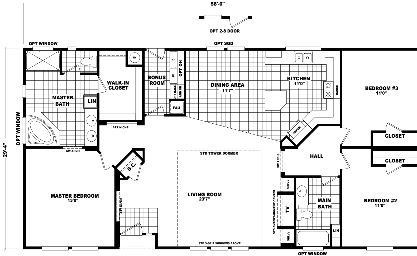
MODEL: EST3058A APPROXIMATELY 1693 SQ. FT. 3 BEDROOM, 2 BATH
