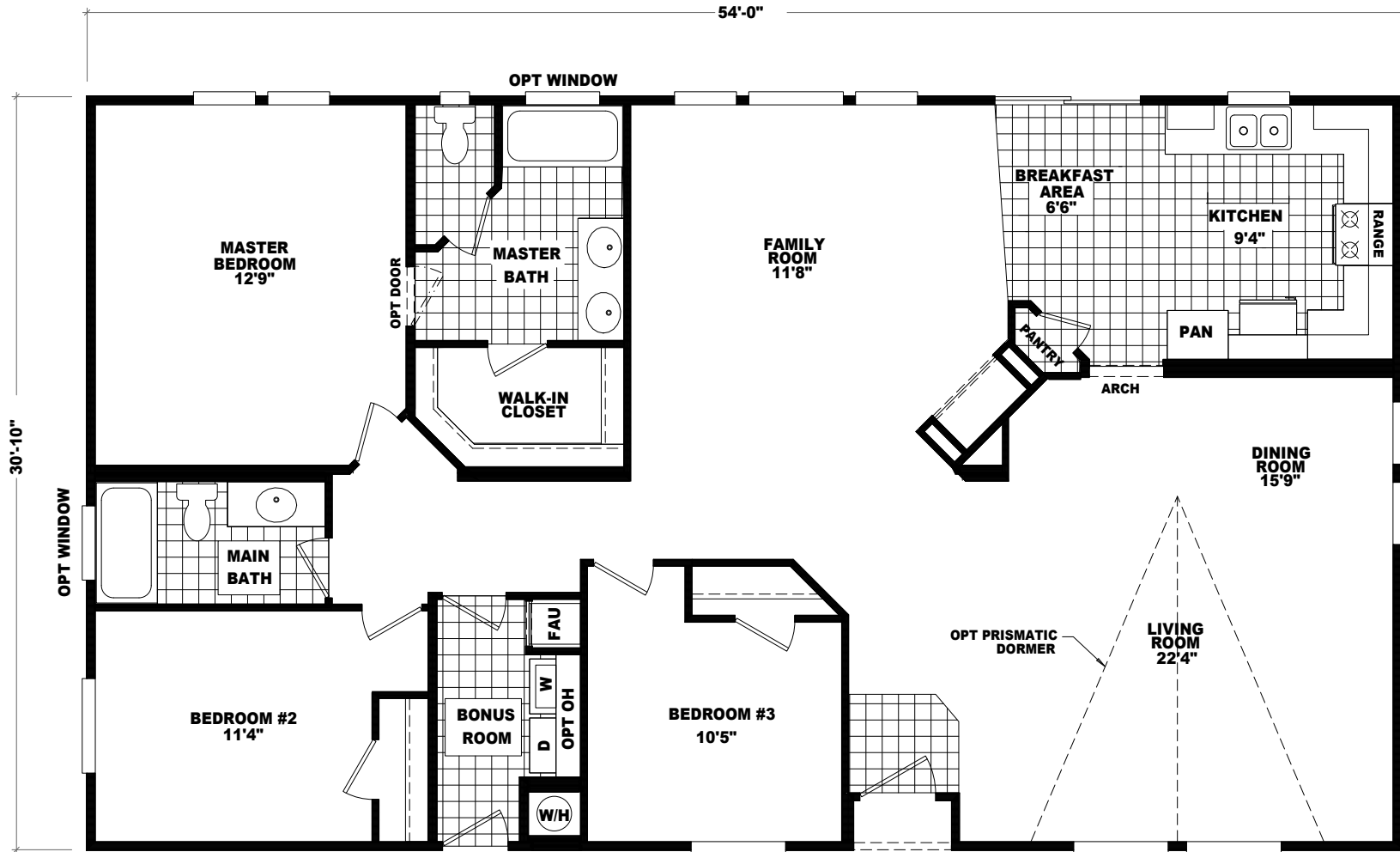
MODEL: DEV-1687A APPROXIMATELY 1665 SQ. FT. 3 BEDROOM, 2 BATH
