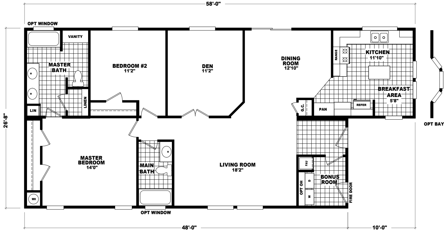
MODEL: DEV-1414A APPROXIMATELY 1413 SQ. FT. 2 BEDROOM, 2 BATH
