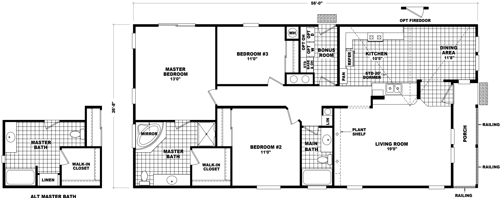
MODEL: DBS-1440A APPROXIMATELY 1440 SQ. FT. 3 BEDROOM, 2 BATH
