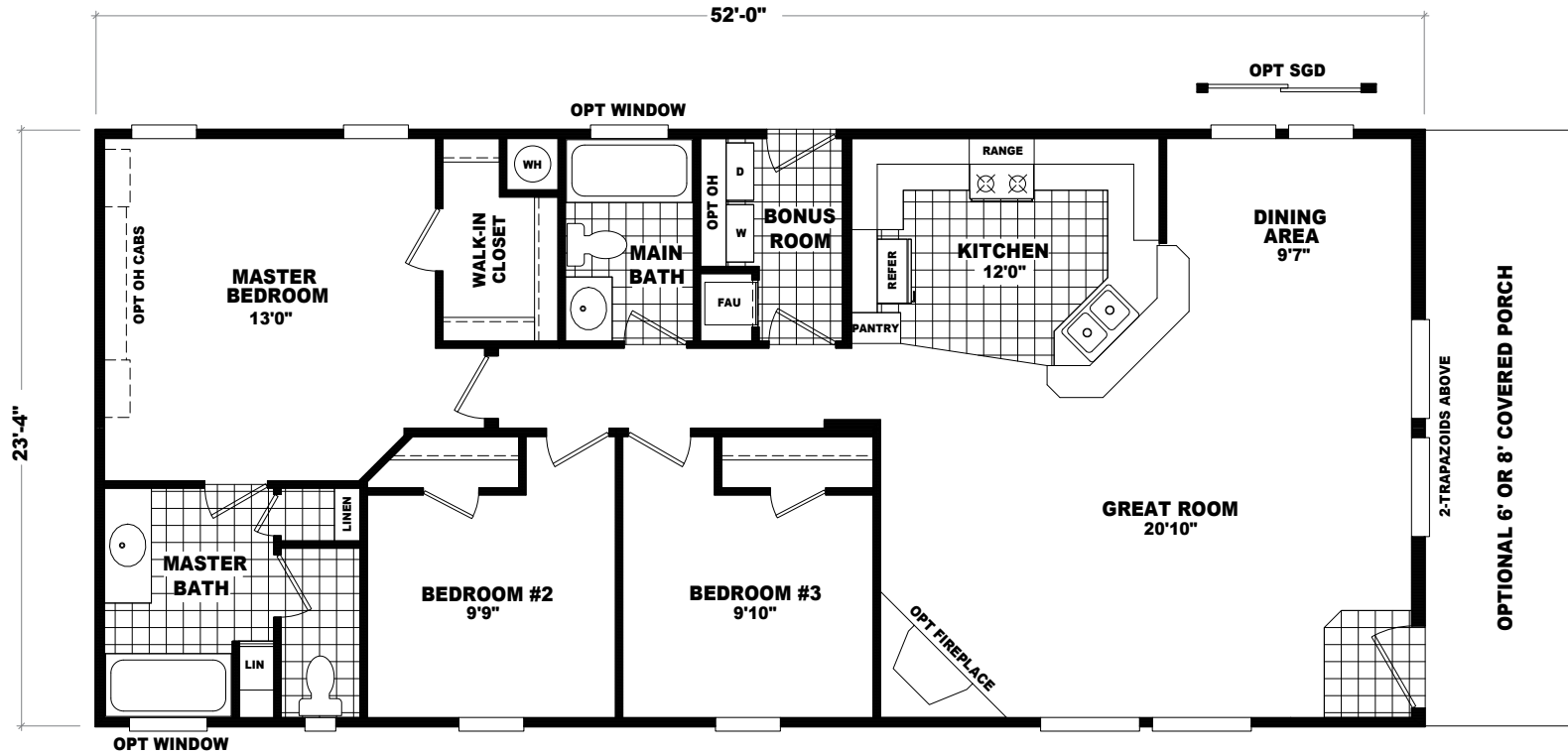
MODEL: CVC2452A APPROXIMATELY 1213 SQ. FT. 3 BEDROOM, 2 BATH
