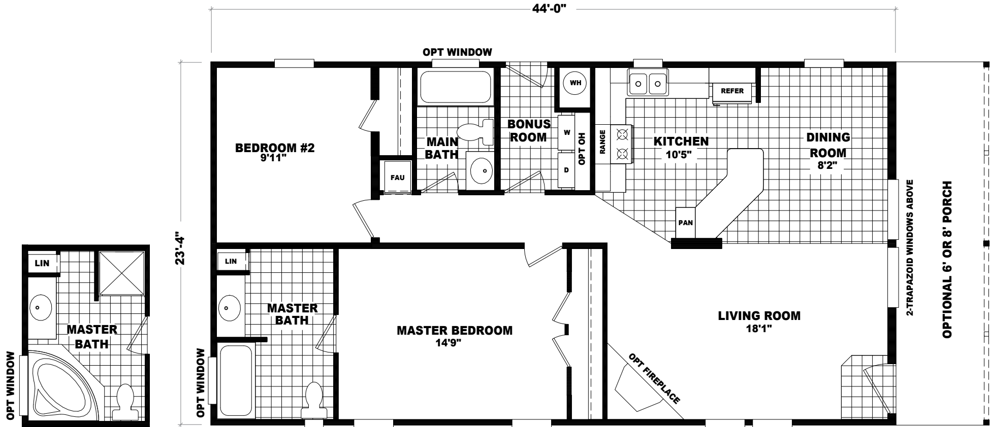
MODEL: CVC2444A APPROXIMATELY 1026 SQ. FT. 2 BEDROOM, 2 BATH
