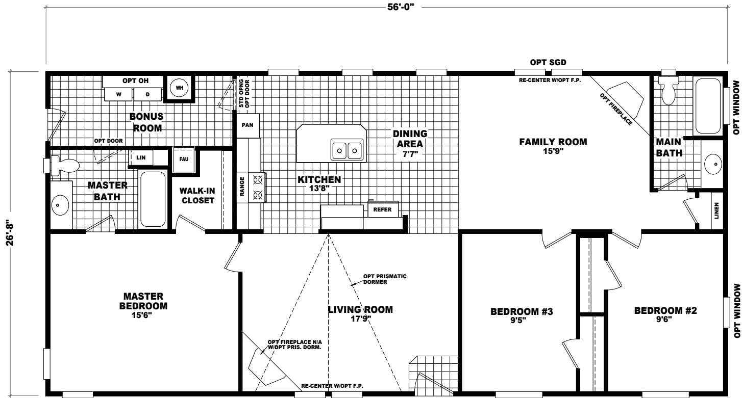
MODEL: CS5628A APPROXIMATELY 1493 SQ. FT. 3 BEDROOM, 2 BATH
