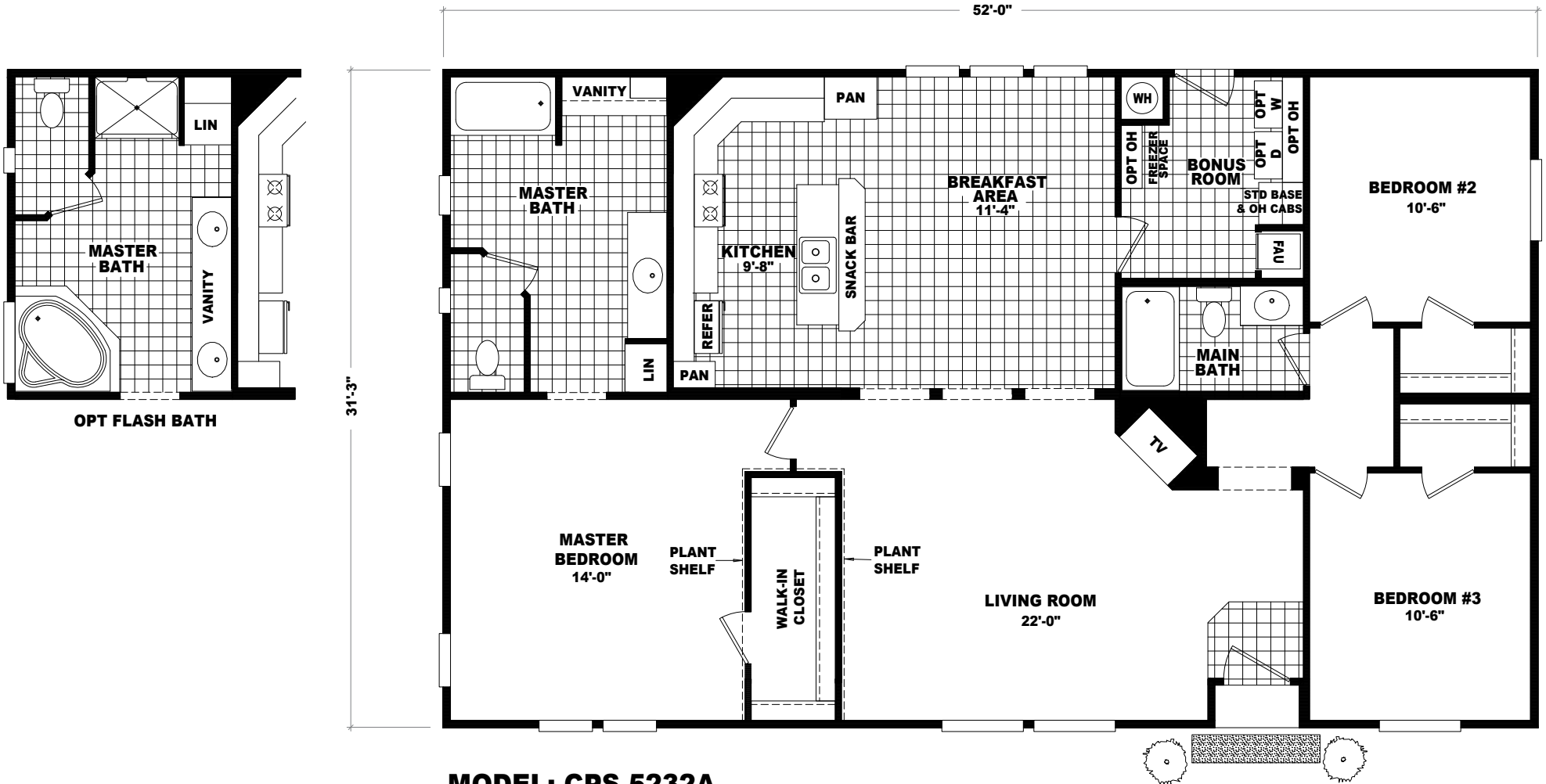
MODEL: CPS-5232A APPROXIMATELY 1625 SQ. FT. 3 BEDROOM, 2 BATH
