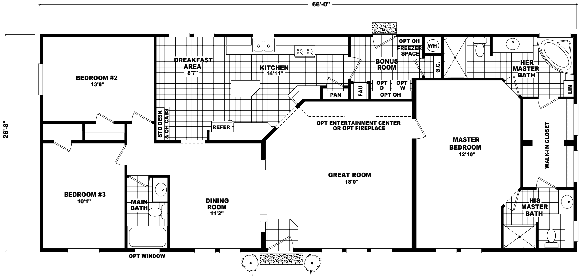
MODEL: CLE-6628A APPROXIMATELY 1760 SQ. FT. 3 BEDROOM, 3 BATH
