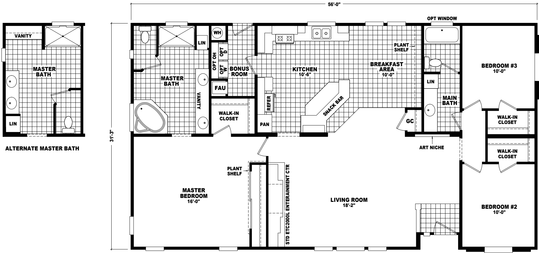
MODEL: ADV-5632A APPROXIMATELY 1750 SQ. FT. 3 BEDROOM, 2 BATH
